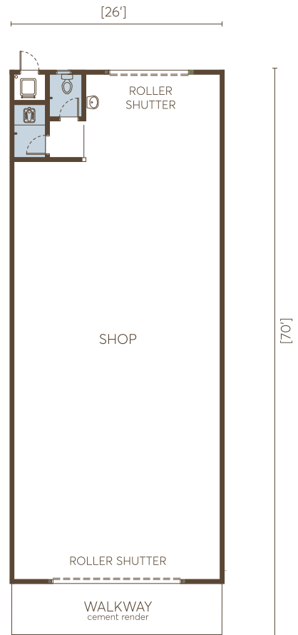
INTERMEDIATE LOT 26' x 70'
